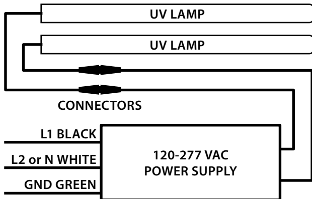
Electrical Diagram
